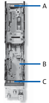
Installation backplane for Single Drive:
